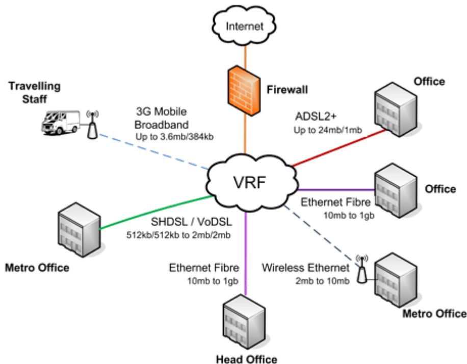
Figure 1: The Genisyst managed MPLS VPN service is available Australia-wide. A schematic representation of an MPLS VPN is shown here.
